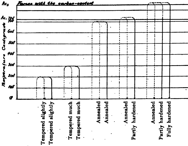
Fig. 73. The Rate of Cooling from below the Transformation Range is Immaterial, from above that Range is Decisive.
